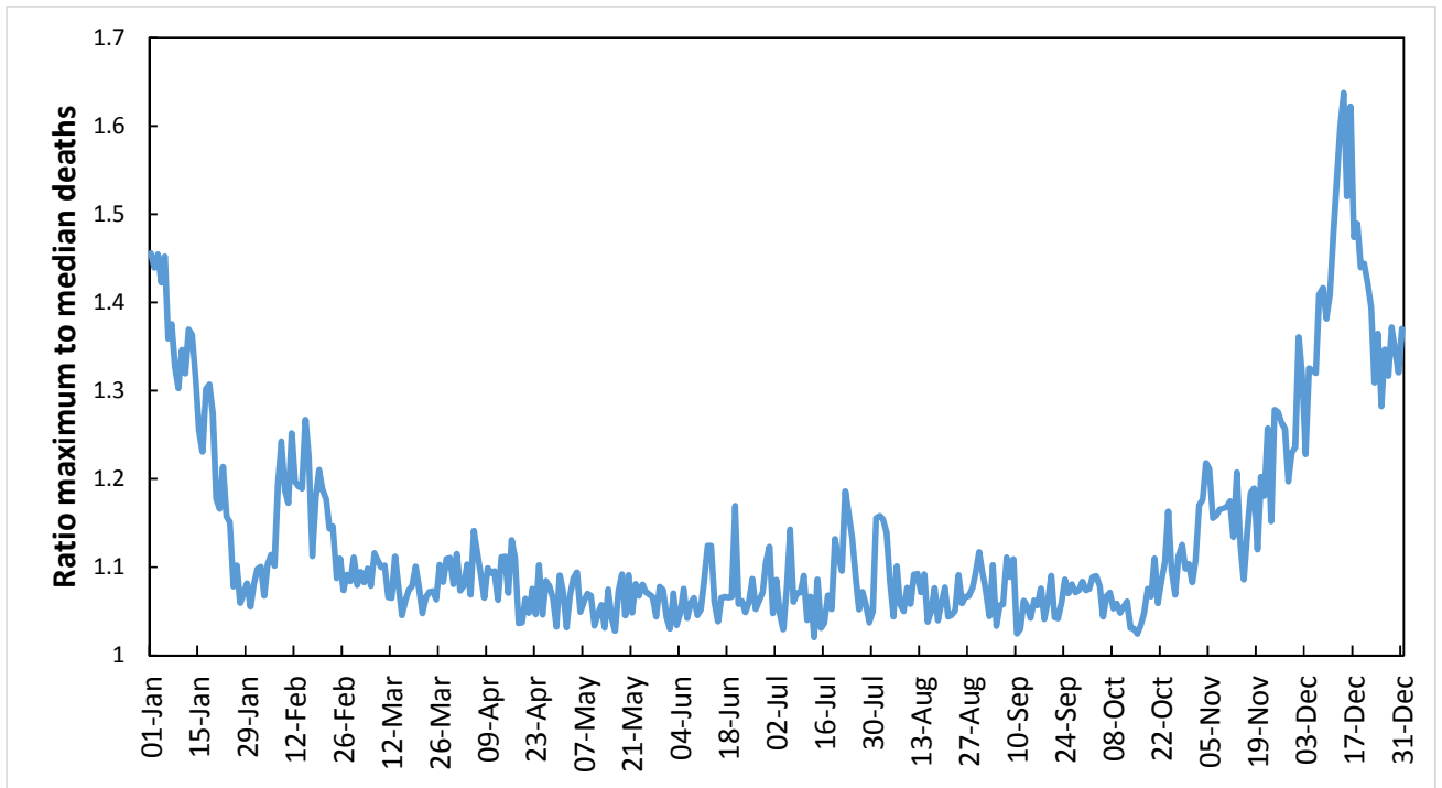
Figure 3: Ratio of daily maximum to median deaths (1989 to 2000) in England & Wales
