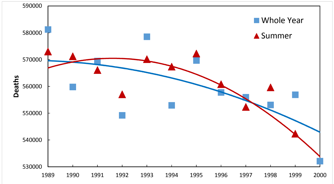
Figure 4: Hypothetical baseline using 'whole year' or 'summer' deaths in England & Wales
