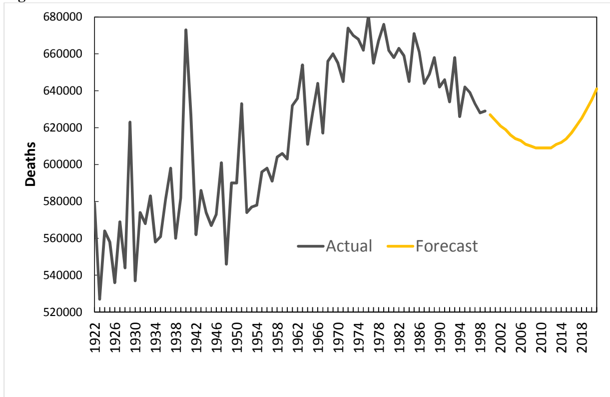
Figure 1: Actual and forecast deaths in the UK
