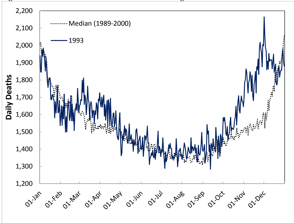
Figure 5: The 1993 outbreak and trends in death for England & Wales
